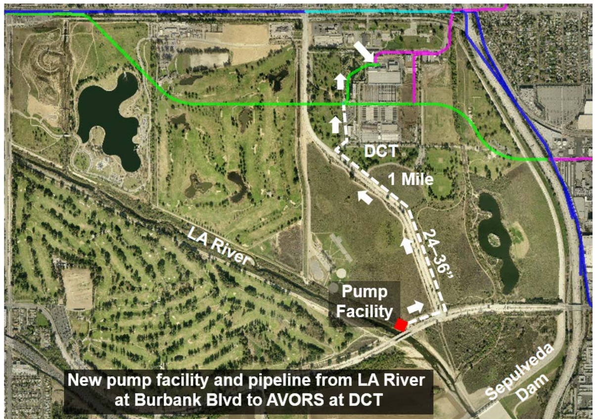
Figure 11 Pump Facility and Pipeline from Sepulveda Dam to DCTWRP
